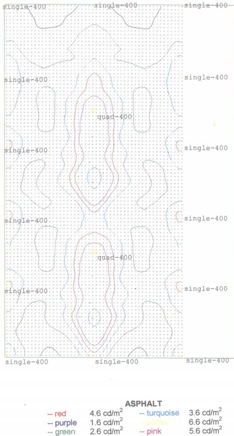
Figure 7b. Iso-luminance diagrams for asphalt parking lot pavement (This was calculated according IES standards. The values were obtained by Lumen Micro 7.5™.)
